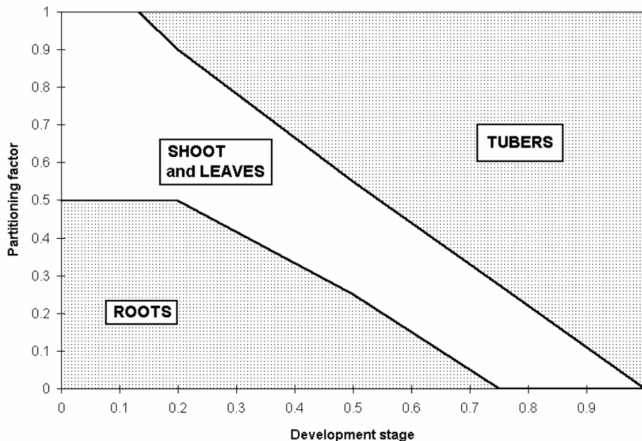
Figure 8: an example of partitioning of biomass in a root crop at different development stages (based on data in McKerron, 1992)
