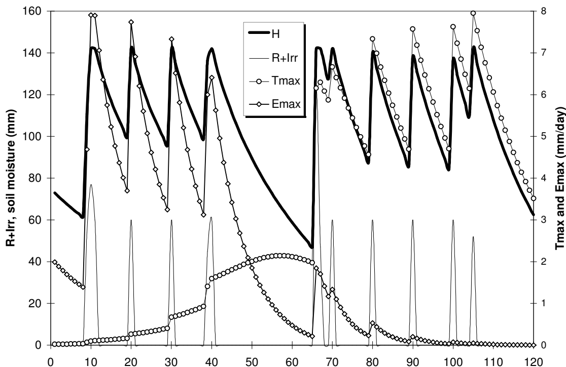
Figure 36: some simulated model variables (soil moisture, water supply as rainfall and irrigation, potential transpiration and potential evaporation).
