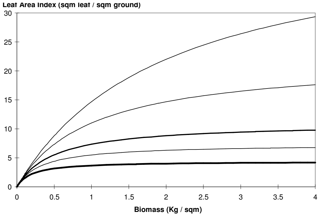
Figure 38 : LAI as a function of biomass for various stem-leaf partitioning factors varying from 0.5 (top) to 1, 2, 3 and 5 m 2 ground / kg biomass (bottom).
