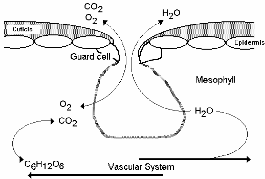
Figure 5: schematic representation of a stomate and the movements of CO 2 , O 2 and H 2 O which take place between leaf and atmosphere.
