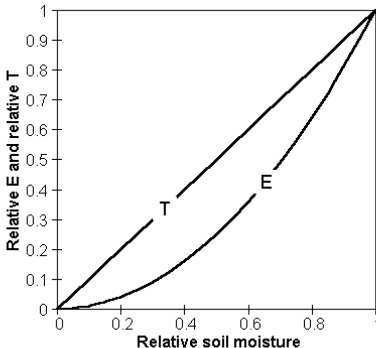
Figure 35 : dependence of relative evaporation and relative transpiration on relative soil moisture for a simple soil water balance simulation with a spreadsheet.
