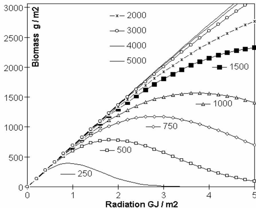
Figure 29 : annual potential biomass according to the Chikugo model as a function of annual radiation and rainfall (mm) varying between 250 and 5000 mm per year
