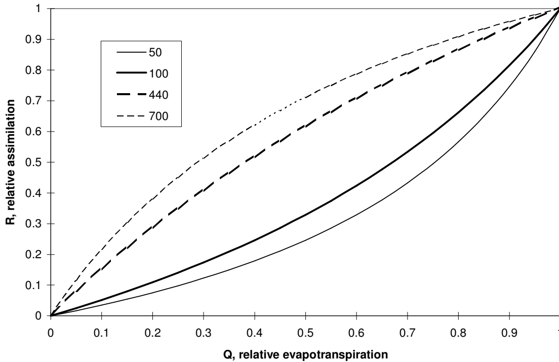
Figure 6 : plot of R versus Q, as function of different mesophyll resistances. r_a was assumed to be 50 \text{ s m}^{-1} .
