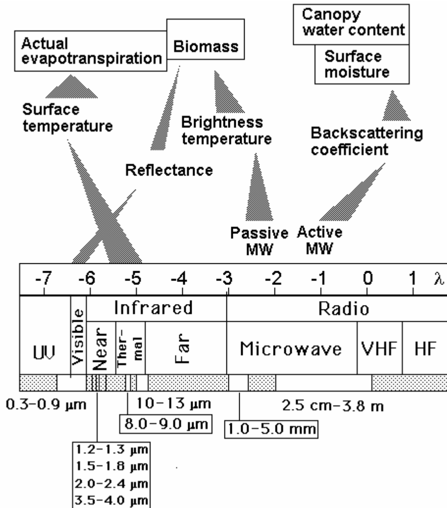
Figure 16 : remote sensing sources of crop weather modelling inputs. \lambda indicates the exponent of the wavelength in m (- 6 corresponds to a \mu\text{m} , -2 to a cm, etc.). The bottom line shows the main atmospheric windows, i.e. parts of the spectrum to which there is little absorption in the atmosphere. The absorption is mainly due to \text{CO}_2 (thermal infrared) and water vapour.
