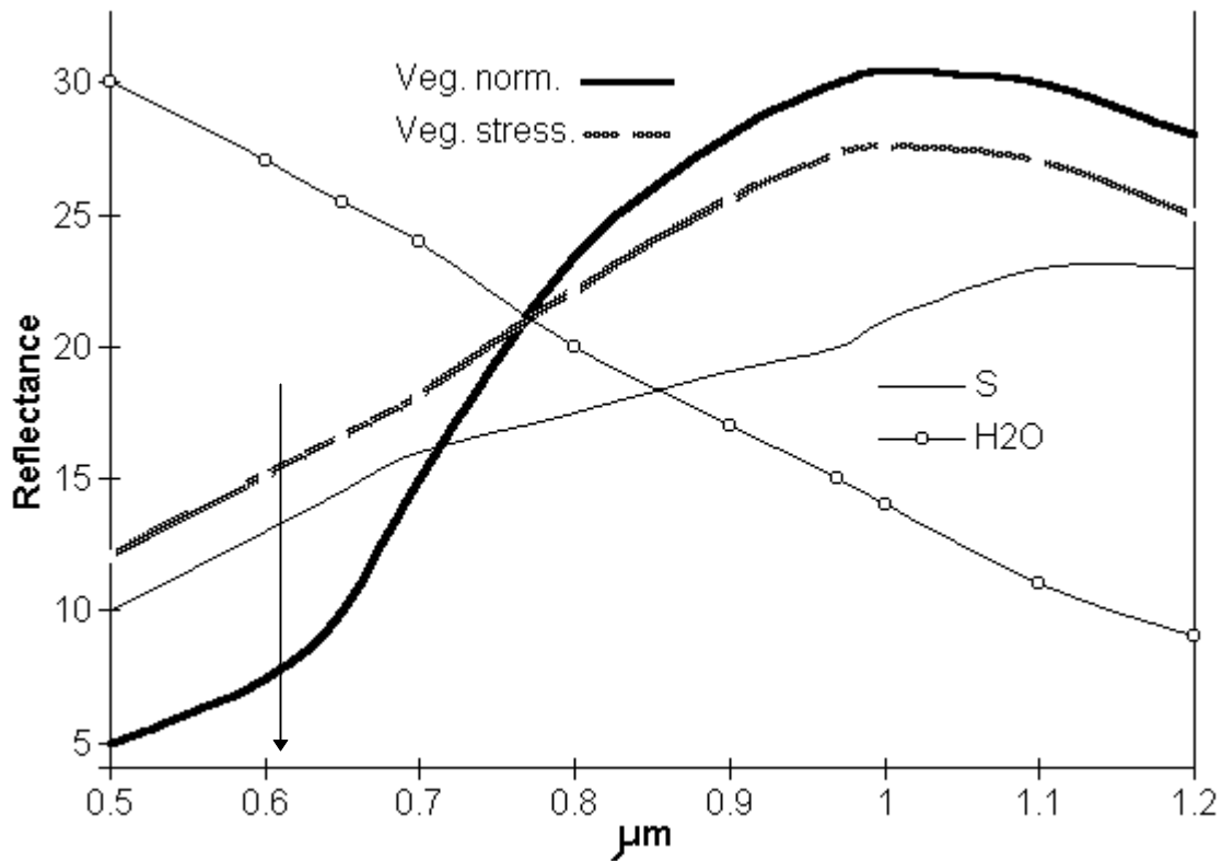
Figure 17 : reflectance spectrum 51 of stressed vegetation , vegetation in good health (veg. Norm), soil (S) and water H 2 O. The arrow indicates the second (red) peak of absorption of chlorophyll.
