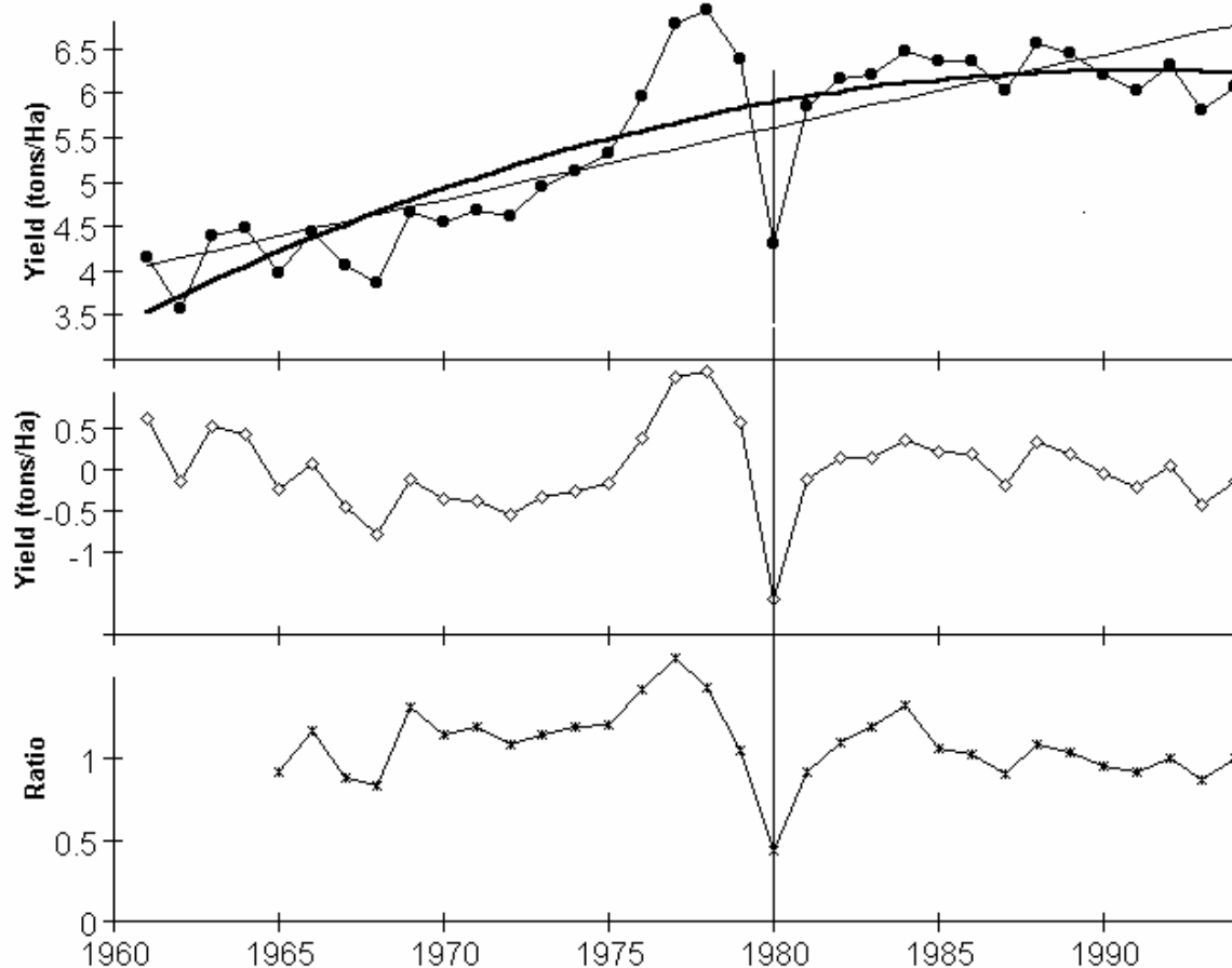
Figure 25 : Yield of total paddy in the Korean Republic between 1960 and 1994 (based on FAO statistics). The top curve indicates the actual yields with their linear and quadratic trends; the middle curve is the detrended yield, i.e. the difference (residual) between actual yield and the quadratic trend; the lower curve shows the ratio between the yield of year N upon the average of the 4 years from N-1 to N-4.
