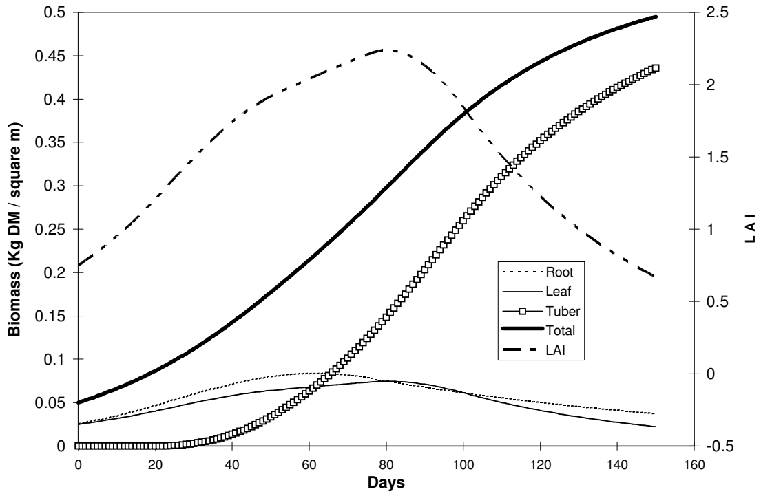
Figure 34 : results of a simple root crop simulation using a spreadsheet.
