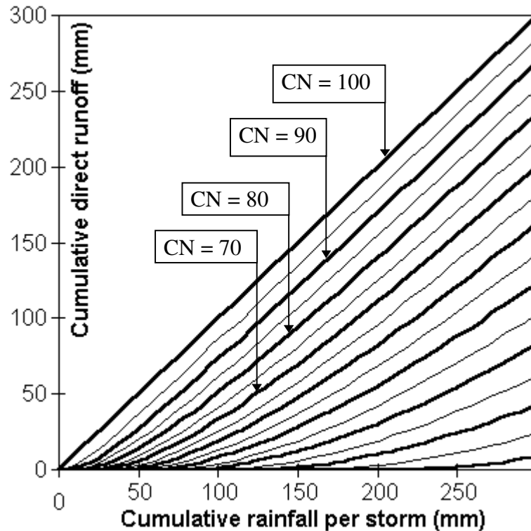
Figure 10 : USDA-SCS relation between storm runoff and rainfall for curve numbers between 100 and 20 (heavy lines). Thin lines indicate the intermediate CN values (95, 85 etc.).
